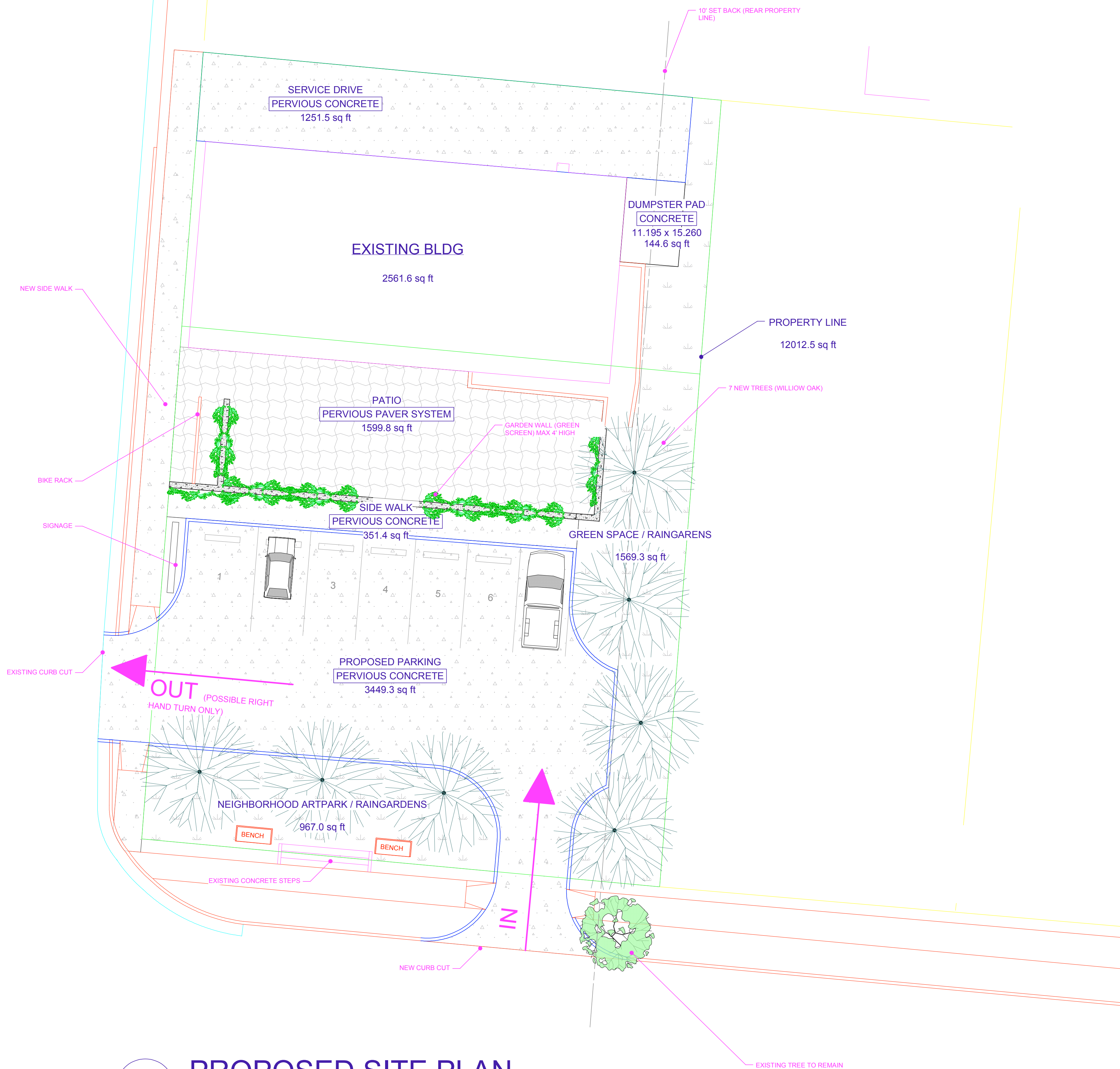
1 PROPOSED SITE PLAN 0 30 36 42 48 54 FT
